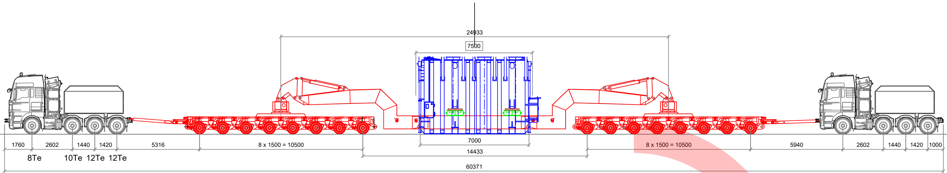
SIDE VIEW 1:150
